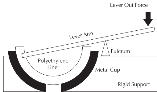
LEVER OUT TEST ASSEMBLY
